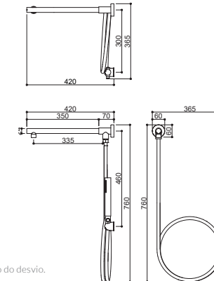
Ref. KR8145 Acabamento rose gold [40999].
